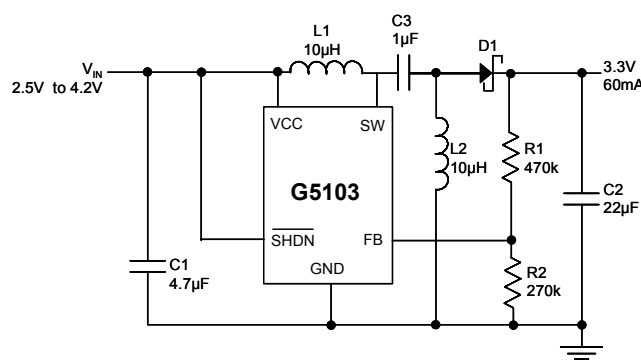
L1,L2:MURATA LQH3C100K24 D1:MOTOROLA MBR0520
