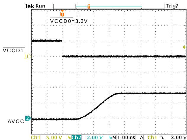
Figure 4. AVCC Propagation Delay and Rise Time With 147 \mu F Load, 3.3V Switch
