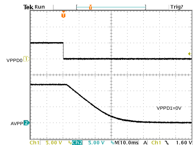
Figure 13. AVPP Propagation Delay and Fall Time With 147 \mu F Load, 12V Switch
