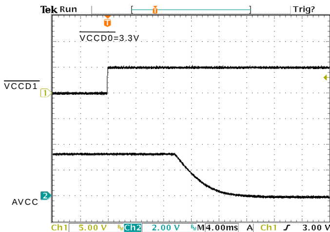
Figure 5. AVCC Propagation Delay and Fall Time With 147 \mu F Load, 3.3V Switch
