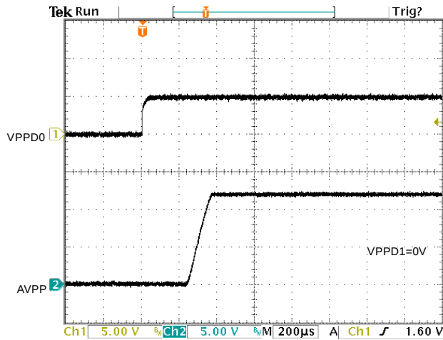
Figure 10. AVPP Propagation Delay and Rise Time With 1 \mu F Load, 12V Switch
