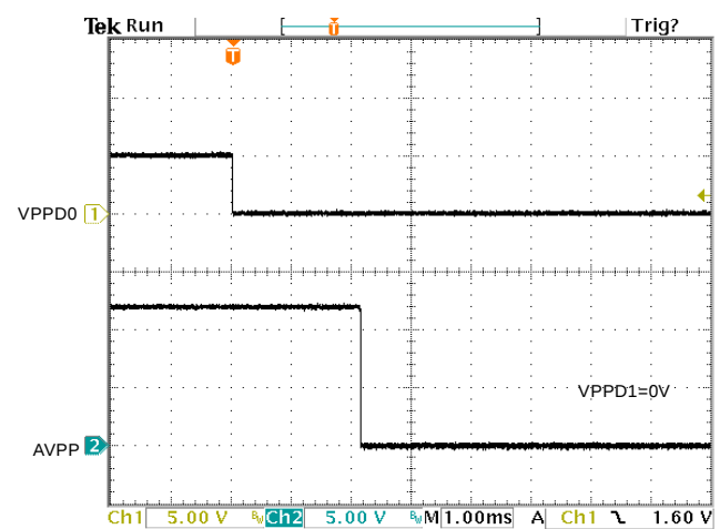
Figure 11. AVPP Propagation Delay and Fall Time With 1 \mu F Load, 12V Switch
