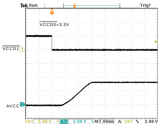
Figure 2. AVCC Propagation Delay and Rise Time With 1 \mu F Load, 3.3V Switch
