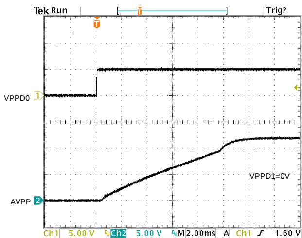
Figure 12. AVPP Propagation Delay and Rise Time With 147 \mu F Load, 12V Switch
