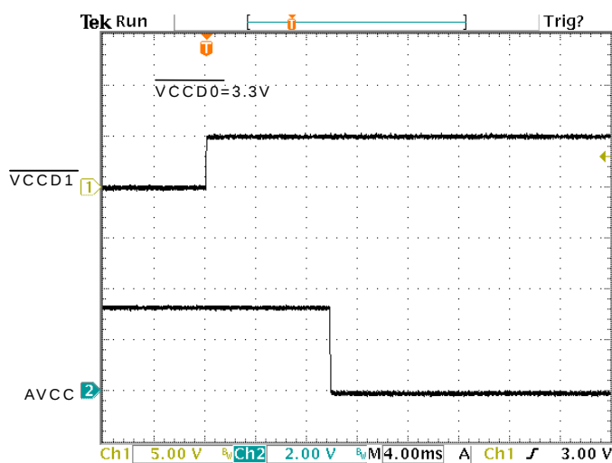
Figure 3. AVCC Propagation Delay and Fall Time With 1 \mu F Load, 3.3V Switch
