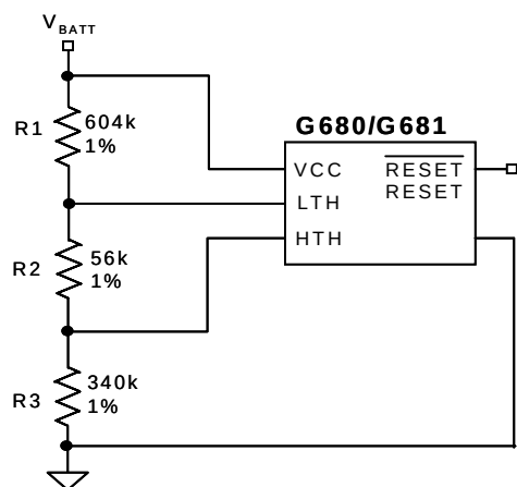
Figure 2. Example Circuit
