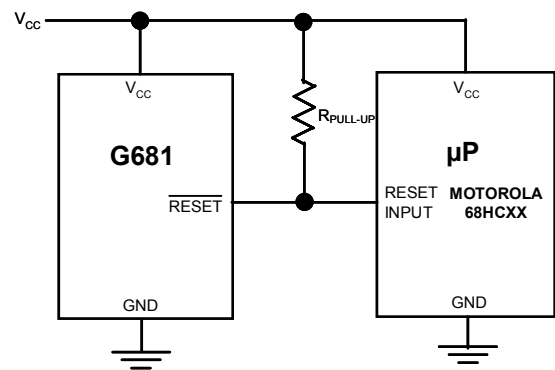
Figure 3. Interfacing to \mu\text{Ps} with Bidirectional Reset I/O
