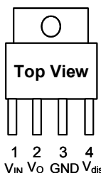
TO-220F-4
