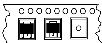
Feed Direction TO252 - 263 Package Orientation
