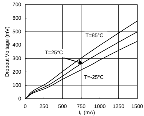
Dropout Voltage vs. I_L (G965-18)
