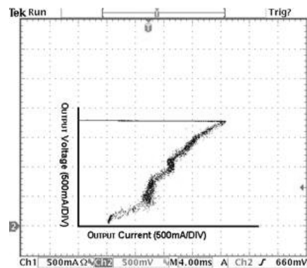
Overcurrent Protection Characteristics(G965-18)
