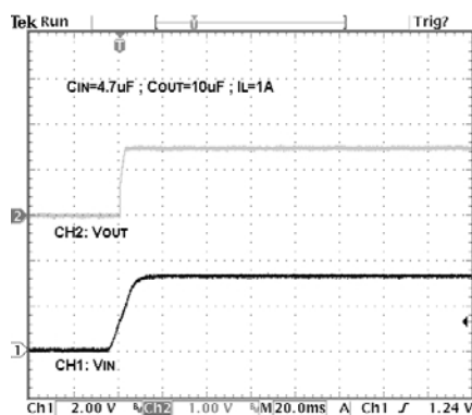
Start-UP(G965-15)
