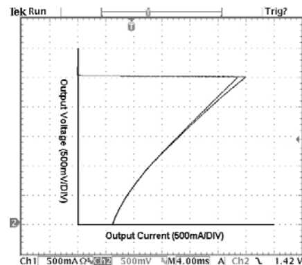
Overcurrent Protection Characteristics(G965-25)
