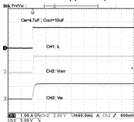
Start-up(G965-25)
