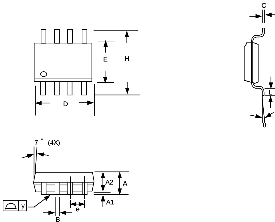
SOP-8 Package
