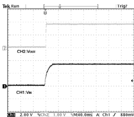
Start-up(G965-18)
