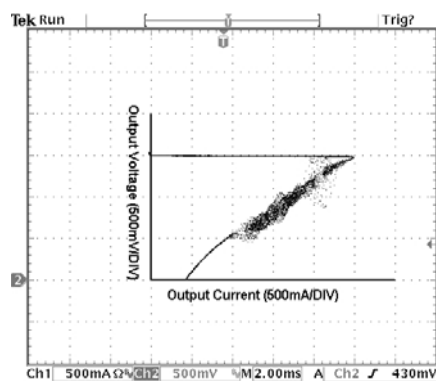
Overcurrent Protection Characteristics(G965-15)
