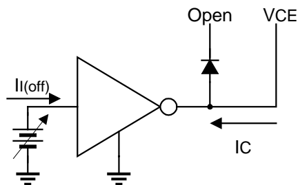
Figure 1 ICEX Test Circuit
