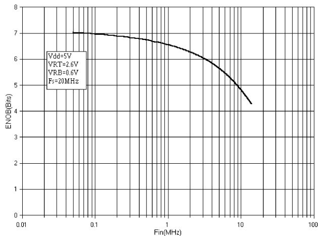
Graph 8. ENOB vs. Input Frequency
