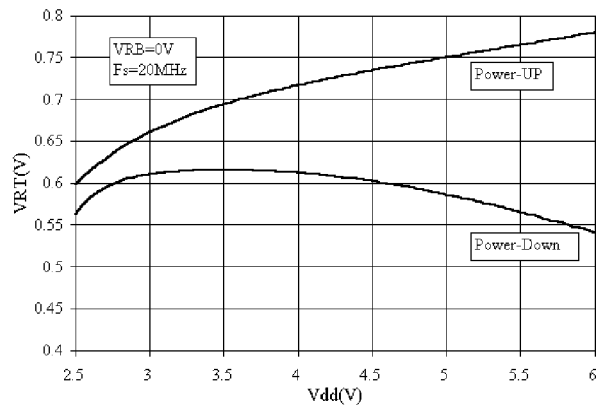
Graph 7. Power Up/Down Voltage vs. Supply Voltage
