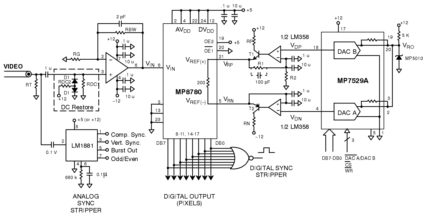
Figure 21. Video Digitizer
