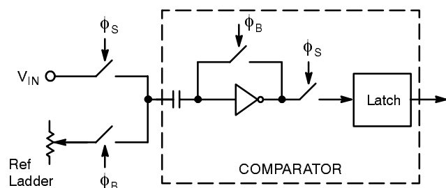
Figure 6. MP8780 Comparator
