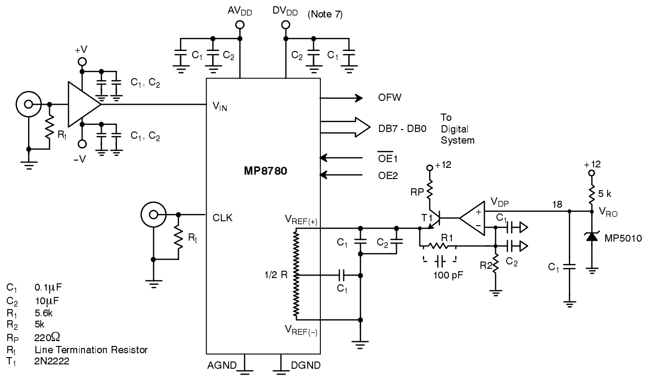
Figure 20. Typical Circuit Connections
