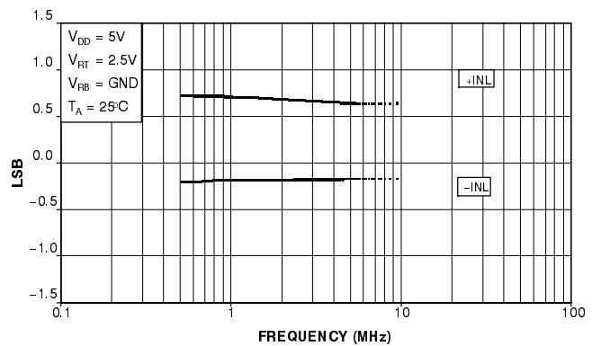
Figure 12. INL vs FREQUENCY
