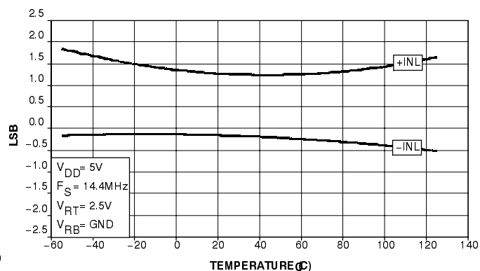
Figure 16. INL vs Temperature
