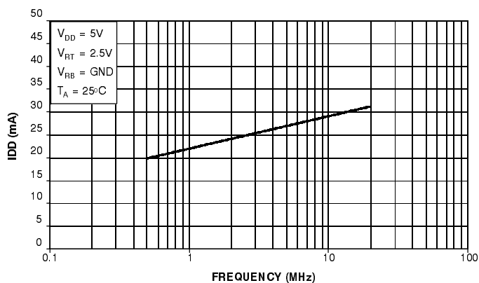
Figure 17. IDD vs FREQUENCY
