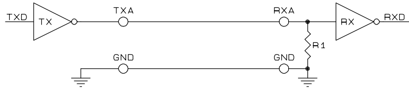
Figure 19. Typical V.10 or V.28 Interface (R1 = 10 K \Omega in V.10 and 5 K \Omega in V.28)
