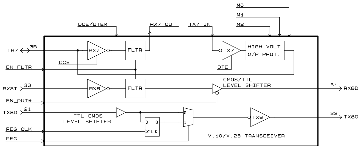
Figure 4. XRT4000 RTMOD3 Block
