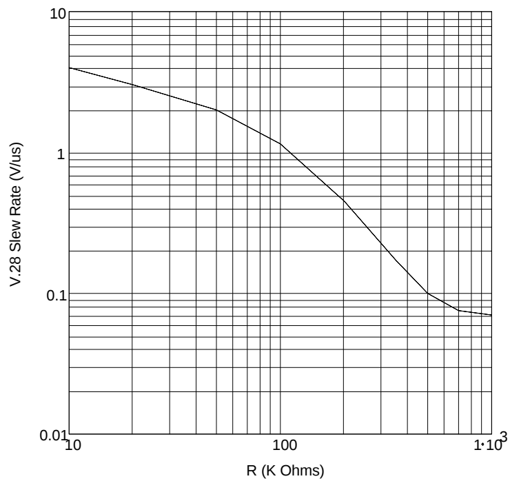
Figure 16. V.28 Slew Rate Over \pm 3 V Output Range with 3\text{ k}\Omega in Parallel with 2500\text{ pF} Load as a Function of RSLEW
