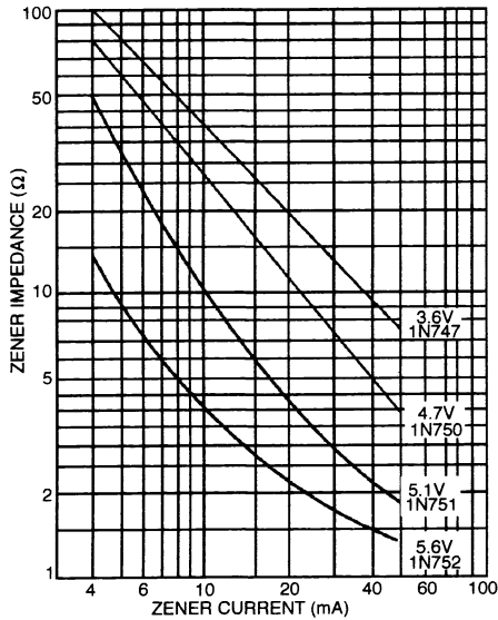
FIGURE 2 ZENER IMPEDANCE VS ZENER CURRENT (TYPICAL)
