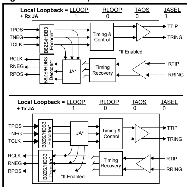
Figure 9: Local Loopback with Selectable JA
