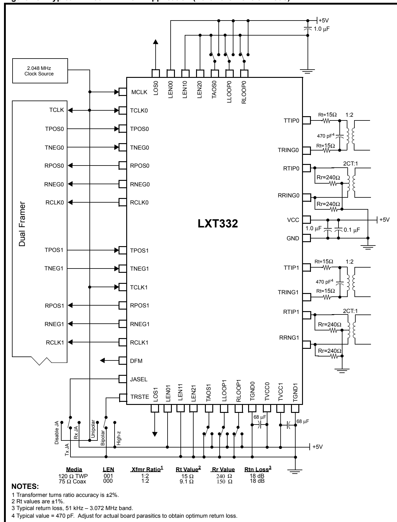
Figure 15: Typical LXT332 E1 120 \Omega Application (Hardware Control Mode)
