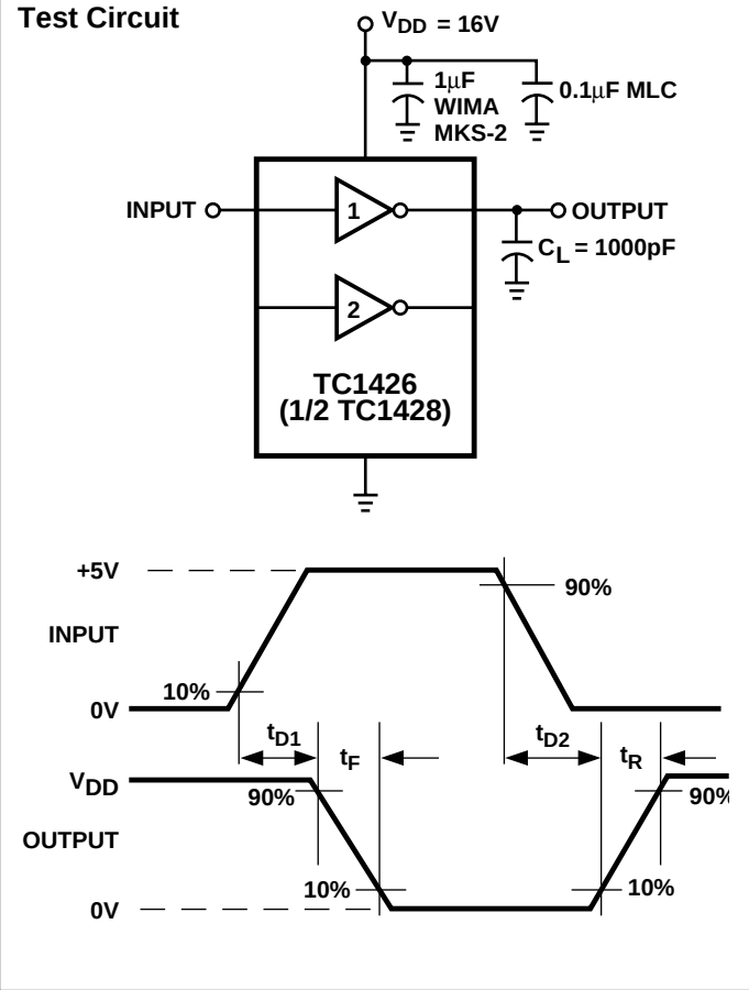
Figure 1. Inverting Driver Switching Time
