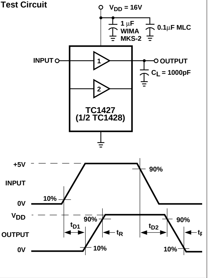
Figure 2. Non-Inverting Driver Switching Time
