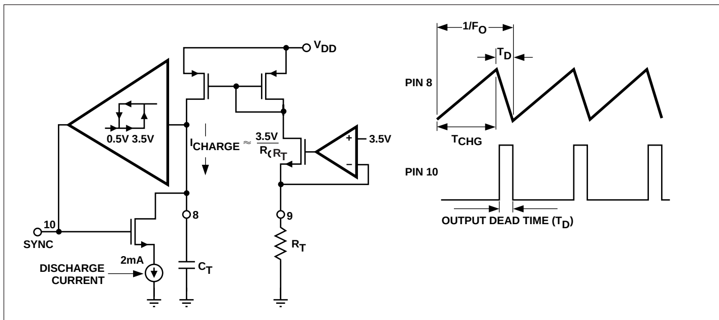
Figure 6. Oscillator Circuit
