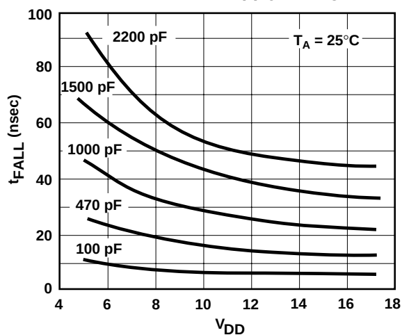
Fall Time vs. Supply Voltage
