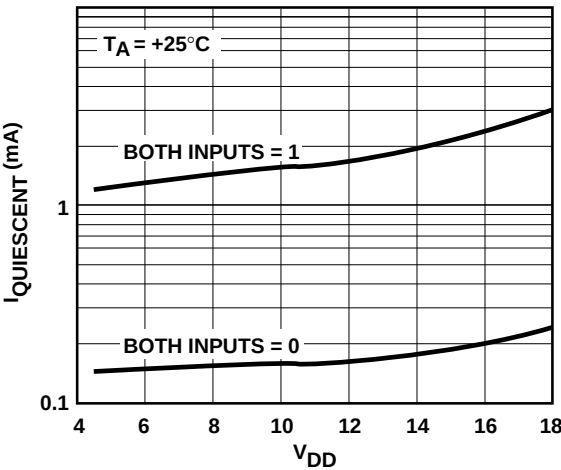
Quiescent Supply Current vs. Voltage
