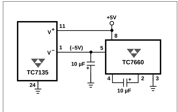
Figure 9. Negative Supply Voltage Generator
