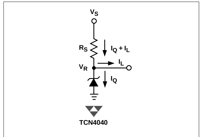
Figure 1. Shunt Regulator
