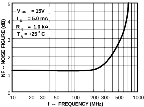
Noise Figure Frequency
