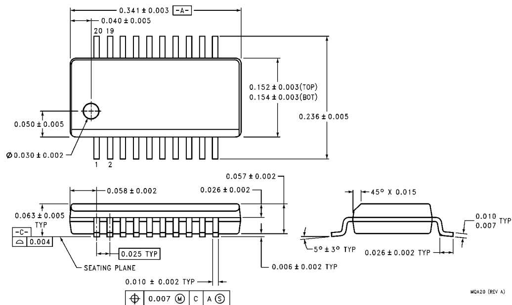
20-Lead Quarter Size Outline Package (QSOP), JEDEC MO-137, 0.150" Wide Package Number MOA20
