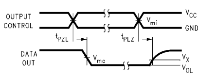
FIGURE 10. 3-STATE Output Low Enable and Disable Times for Low Voltage Logic
