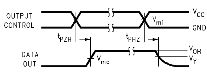
FIGURE 9. 3-STATE Output High Enable and Disable Times for Low Voltage Logic
