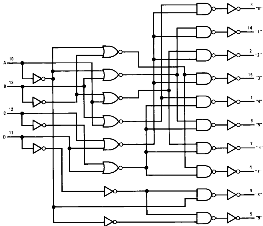
Logic Diagram
