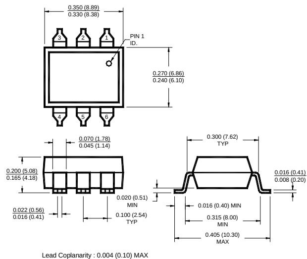
Package Dimensions (Surface Mount)
