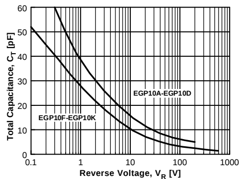
Figure 5. Total Capacitance
