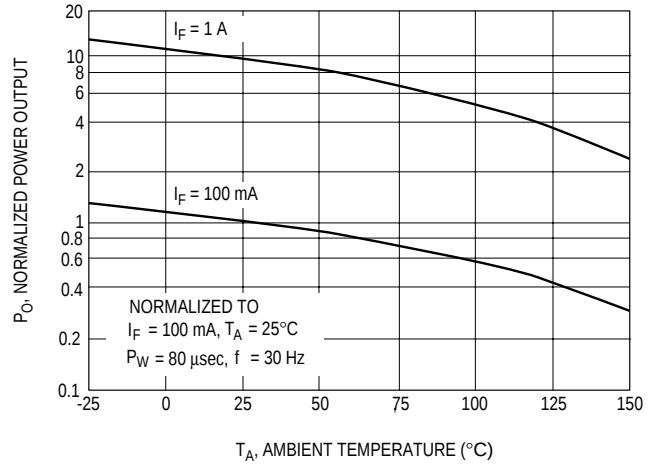
Figure 2. Power Output vs. Temperature
