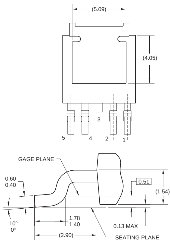
DETAIL A (ROTATED 90°) SCALE: 2X
