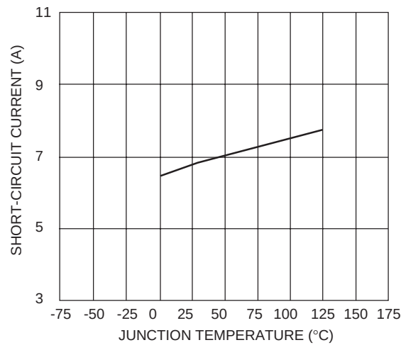
Short-Circuit Current vs. Temeperature
