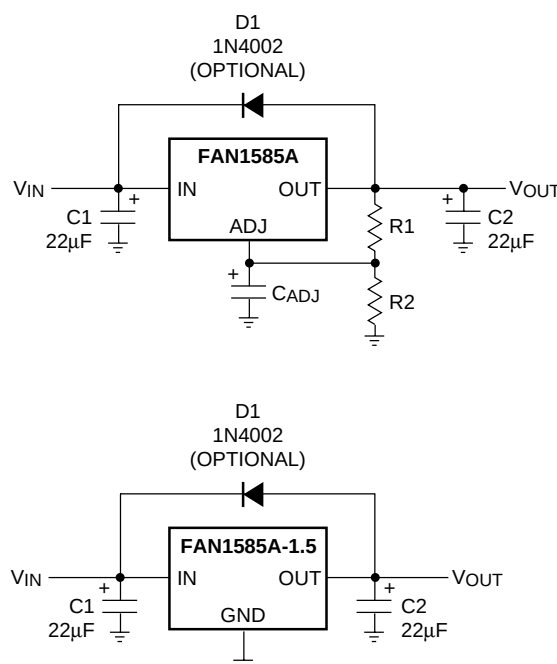
Figure 10. Optional Protection
