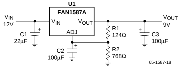
Figure 15. Application Circuit (FAN1587A)
