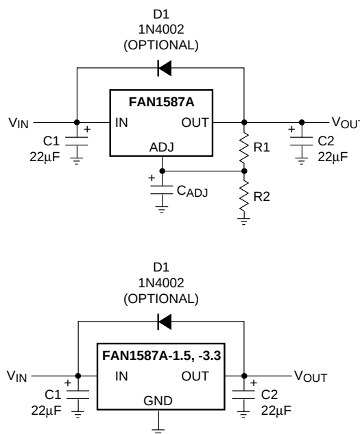
Figure 11. Optional Protection
