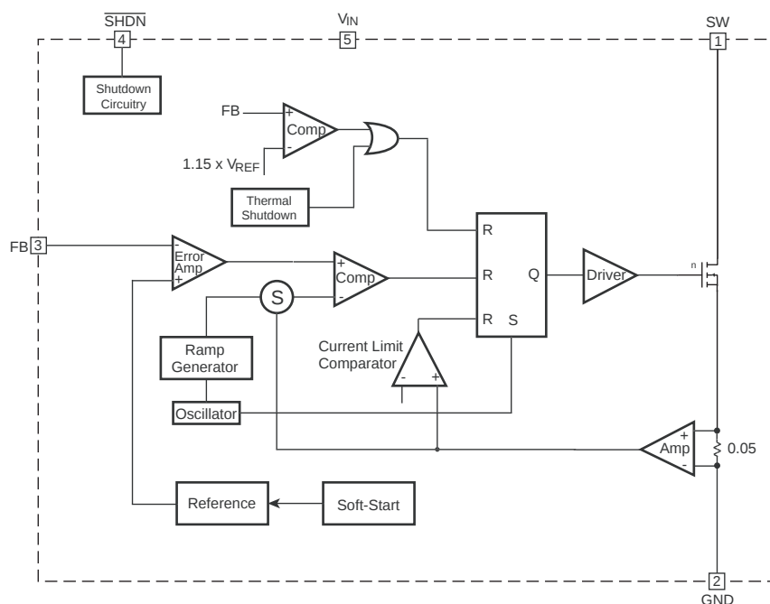
Figure 4. Block Diagram
