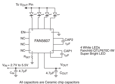
Figure 1. Test Circuit
