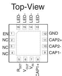
FAN5607 4x4mm 16-Lead MLP
