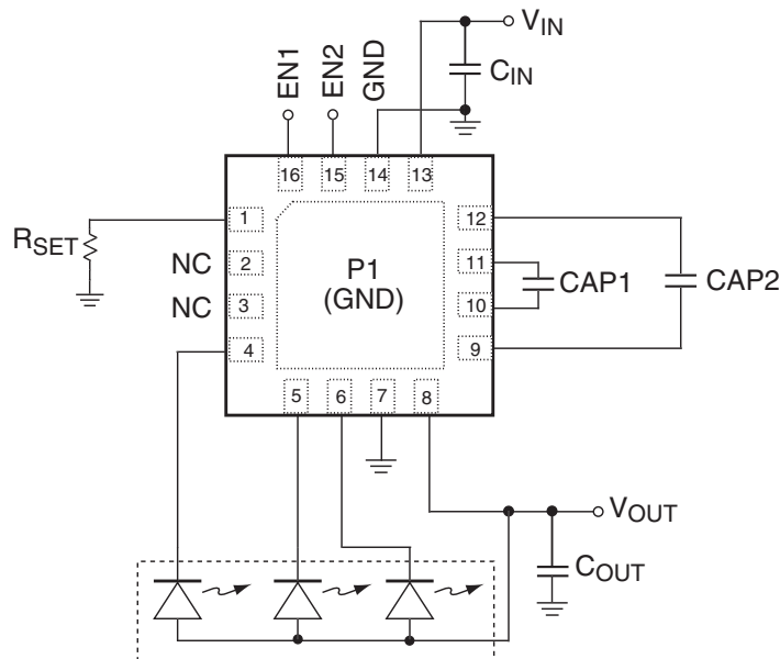
Figure 1. Typical Application
