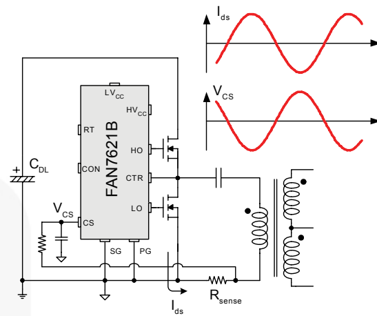
Figure 26. Full-Wave Sensing
