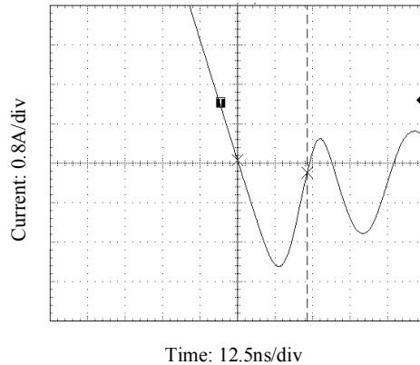
Figure 13. Non-SyncFET (FDP6644) body diode reverse recovery characteristic.
