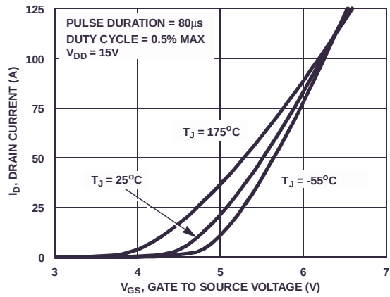
Figure 6. Transfer Characteristics
