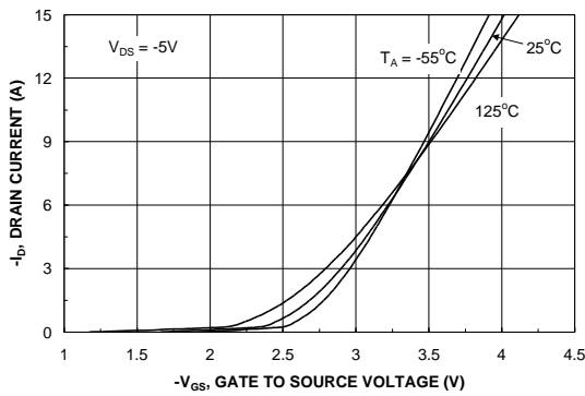
Figure 15. Transfer Characteristics.
