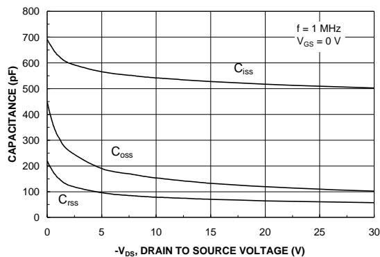
Figure 18. Capacitance Characteristics.
