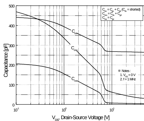
Figure 5. Capacitance Characteristics
