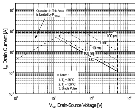
Figure 9-1. Maximum Safe Operating Area for FQP2N50C
