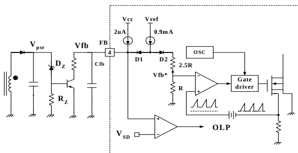
2. Feedback Control : FS8S0765RCB employs primary side regulation, which permits elimination of feedback circuit components in the secondary side such as opto coupler and TL431. Figure 2 shows the primary side control circuit. The primary side regulation voltage ( V_{psr} ) is controlled to the breakdown voltage of zener diode ( D_z ). Because current mode control is employed, the drain current of the power MOSFET is limited by the inverting input of PWM comparator ( V_{fb*} ). When MOSFET turns on, usually there exists high current spike in the MOSFET current caused by primary-side capacitance and secondary-side rectifier reverse recovery. In order to prevent premature termination of the switching pulse due to the current spike, the FPS employs leading edge blanking (LEB). The leading edge blanking circuit inhibits the PWM comparator for a short time after the MOSFET is turned on.
