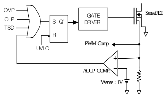
3.1 Abnormal Over Current Protection (AOCP) : When the secondary rectifying diodes or the transformer pins are shorted, a steep current with extremely high di/dt can flow during the LEB time. Therefore, the abnormal over current protection (AOCP) block is added to ensure the reliability as shown in figure 4. It turns off the SenseFET within 300ns after the abnormal over current condition is sensed.
