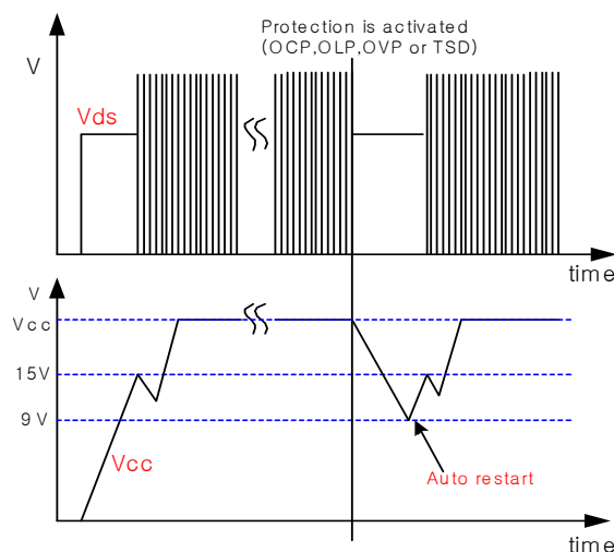
3. Protection function : FS8S0765RCB has 4 self protective functions such as abnormal over current protection (AOCP), over load protection (OLP), over voltage protection (OVP) and thermal shutdown (TSD). Because these protection circuits are fully integrated into the IC without external components, the reliability can be improved without cost increase. In the event of these fault conditions, the FPS enters into auto-restart operation. Once the fault condition occurs, switching operation is terminated and MOSFET remains off, which forces V_{cc} to be reduced. When V_{cc} reaches 9V, the protection is reset and the supply current reduces to 80 \mu A. Then, V_{cc} begin to increase with the current provided through the start-up resistor. When V_{cc} reaches 15V, the FPS resumes its normal operation if the fault condition is removed. In this manner, the auto-restart alternately enables and disables the switching of the power MOSFET until the fault condition is eliminated as illustrated in figure 3.
