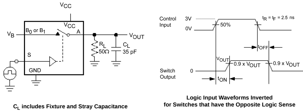
FIGURE 1. Turn-On/Turn-Off Timing
