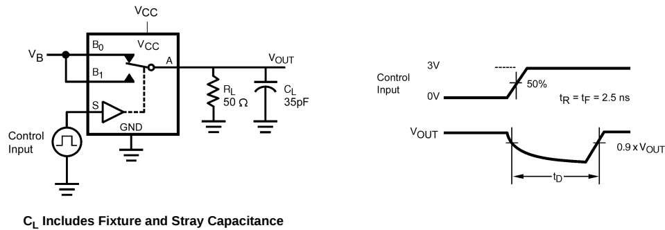
FIGURE 2. Break-Before-Make Timing
