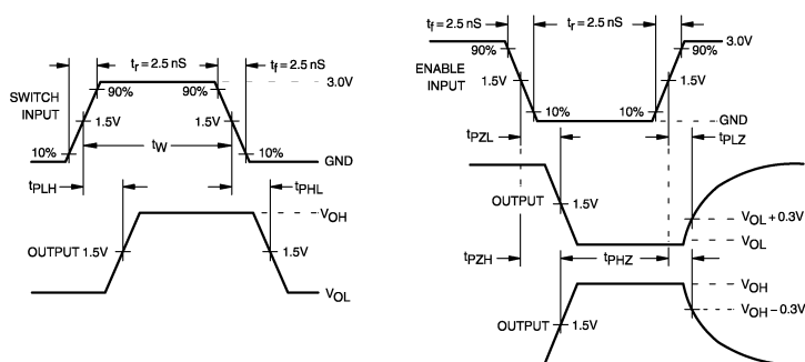
FIGURE 2. AC Waveforms
