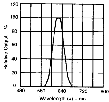
Fig. 2. Spectral Response
