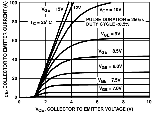
FIGURE 2. SATURATION CHARACTERISTICS
