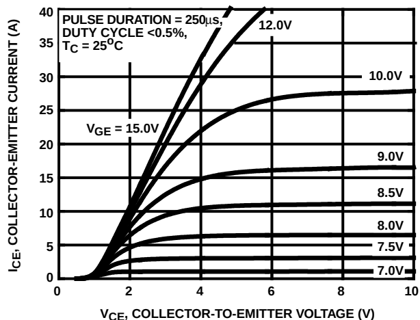
FIGURE 2. SATURATION CHARACTERISTICS
