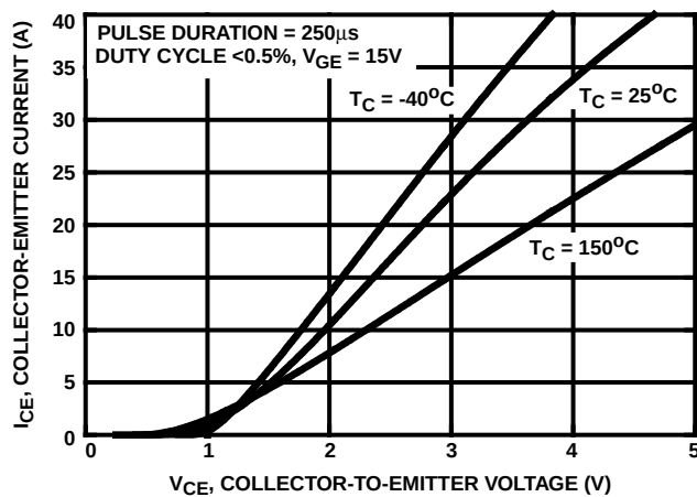
FIGURE 4. COLLECTOR-EMITTER ON - STATE VOLTAGE
