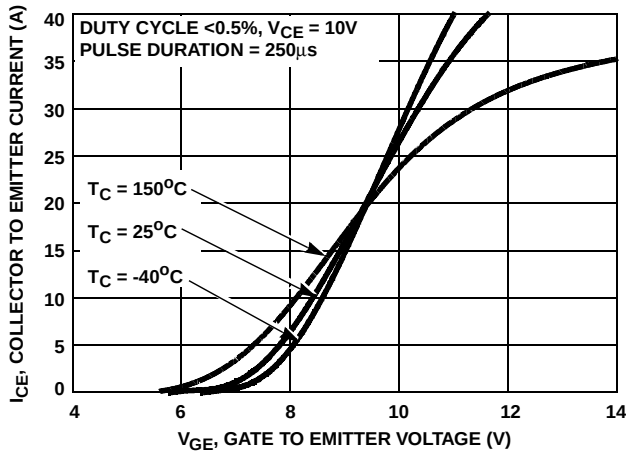
FIGURE 1. TRANSFER CHARACTERISTICS
