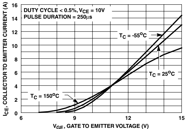
FIGURE 13. TRANSFER CHARACTERISTIC
