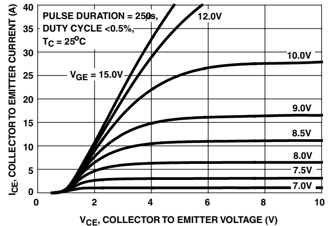
FIGURE 2. SATURATION CHARACTERISTICS
