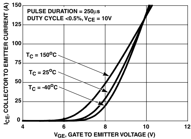
FIGURE 1. TRANSFER CHARACTERISTICS
