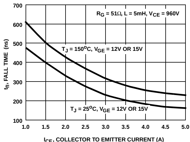
FIGURE 12. FALL TIME vs COLLECTOR TO EMITTER CURRENT
