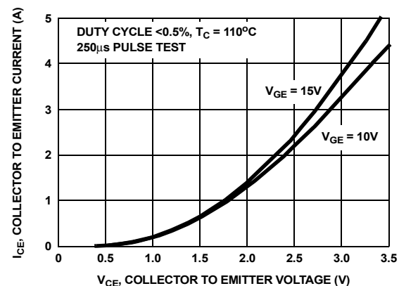
Figure 16. Collector to Emitter On-State Voltage
